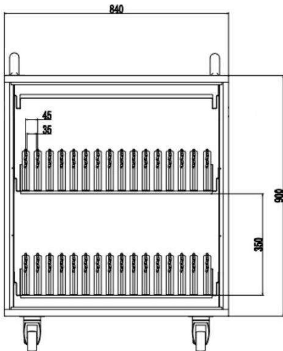
VISTA FRONTAL
