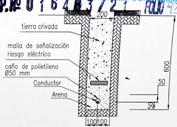
1 CONDUCTOR
