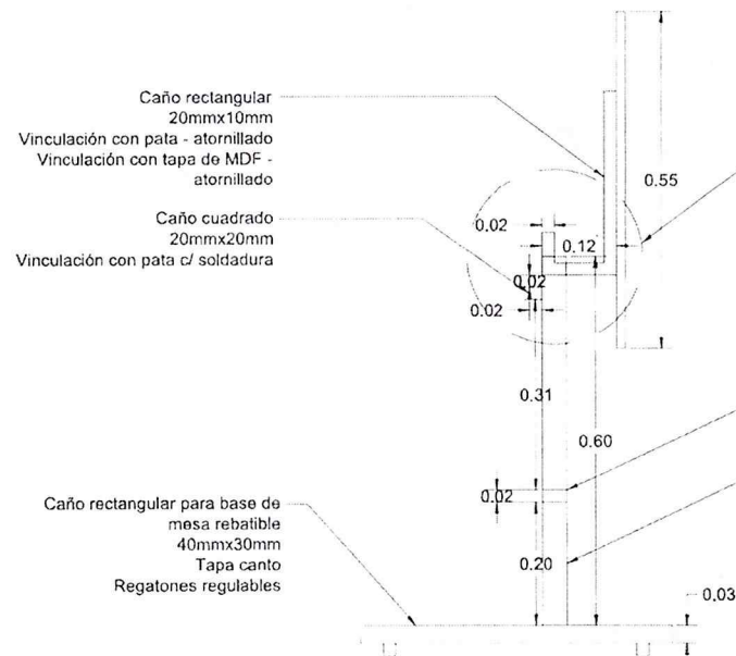
VISTA LATERAL MESA REBATIBLE
