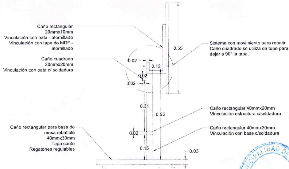
VISTA LATERAL MESA REBATIBLE
