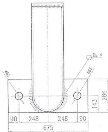
VISTA FRONTAL
